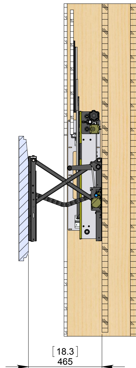
ADVANCE BRACKET SERVICE MODE
