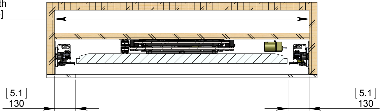
SECTION C-C SCALE 1 : 12
