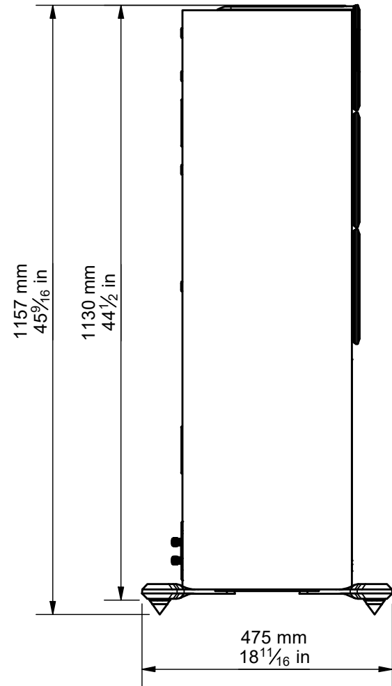
SIDE - GRILLE ON
